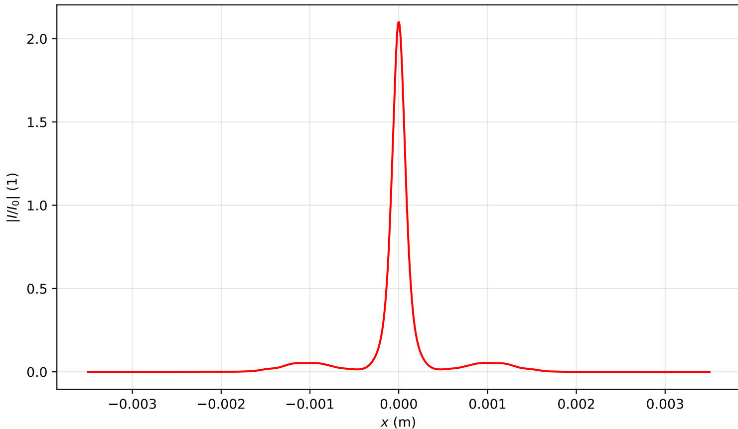
Intensity profile I(x, y = 0, z = 2.627)/I_0 , P_{in}=8.0P_{cr} , artificial time
